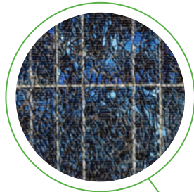
Solder bond failures and cracks in solar cells caused by temperature cycles Repair Cost: $3,500 GGM SunSure Plus: $0
